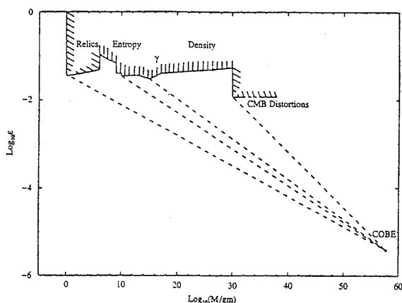
FIG. 2: Constraints on \epsilon(M)
