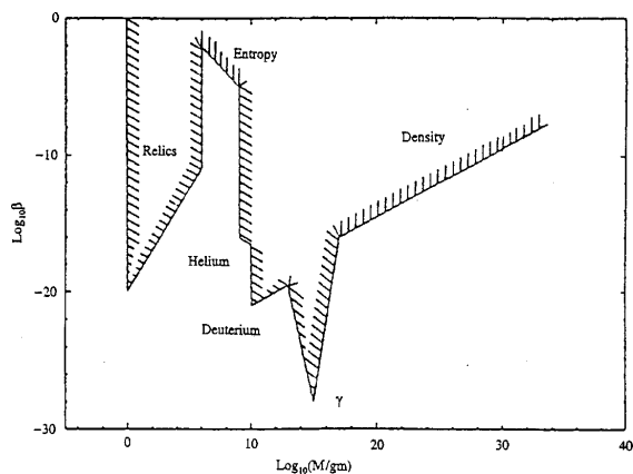
FIG. 1: Constraints on \beta(M)
