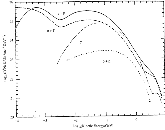
FIG. 4: Instantaneous emission from a 1 GeV black hole
