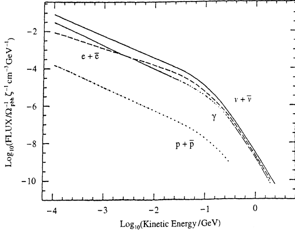
FIG. 5: Spectrum of particles from uniformly distributed PBHs
